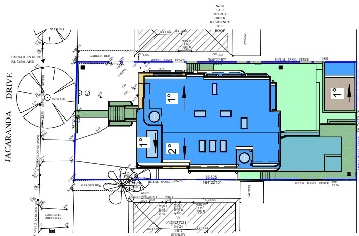
PROPOSED SITE & ROOF PLAN
