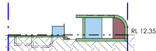
PROPOSED CABANA SOUTH ELEVATION
